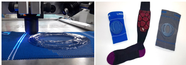
3D printing with simultaneous UV curing (l.), project demonstrators (r.)
