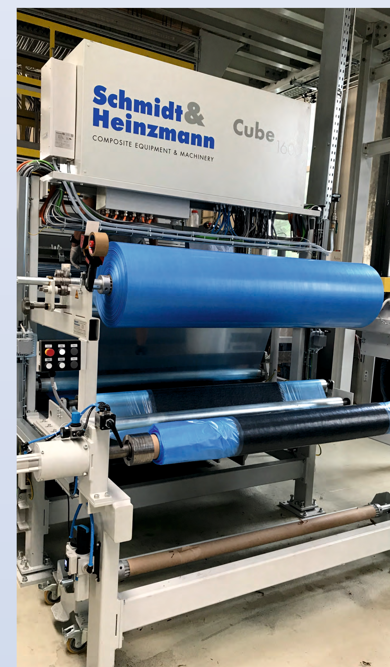
Figure 5: SMC roll good based on carbon fiber nonwoven (© STFI)
